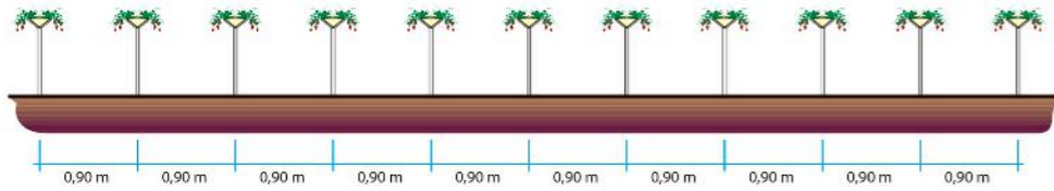
FIXED SYSTEM 100.000 plants/ha
